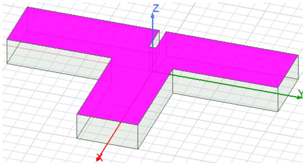
Figure 5-6: Top Face of Tee Selected
